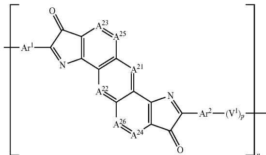
Formula (2-7)
