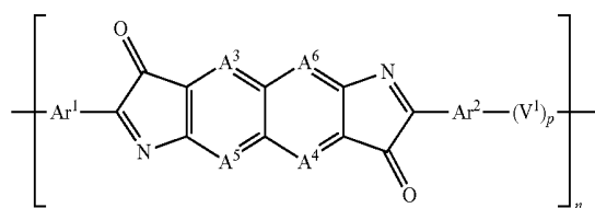
Formula (2-3)
