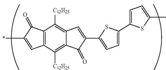
Comparative compound 3
