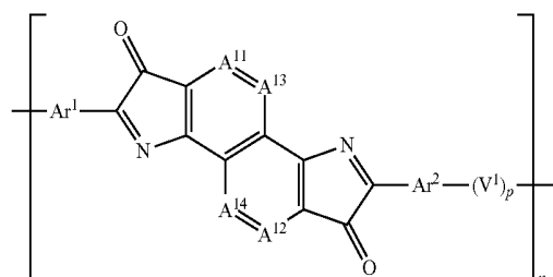
Formula (2-5)
