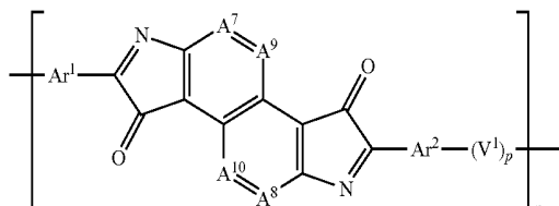
Formula (2-4)
