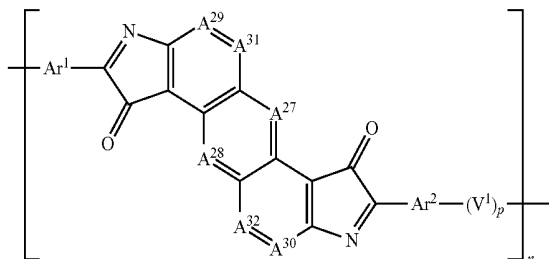
Formula (2-7)
