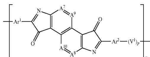
Formula (2-4)
