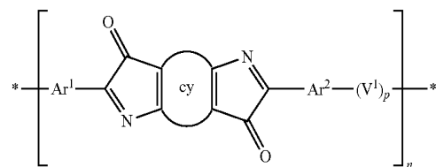
Formula (1-2B)
