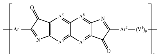
Formula (2-2)
