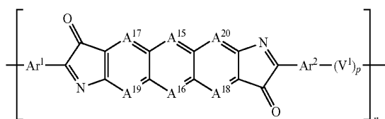
Formula (2-5)
