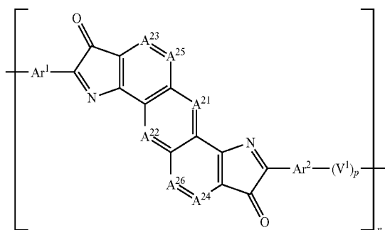
Formula (2-6)
