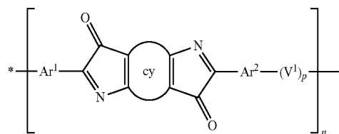
Formula (1-2B)
