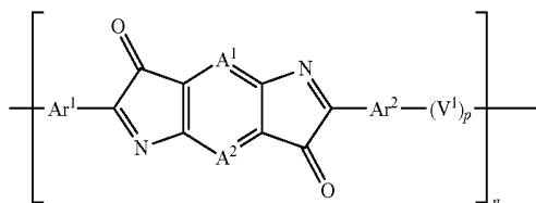
Formula (2-2)
