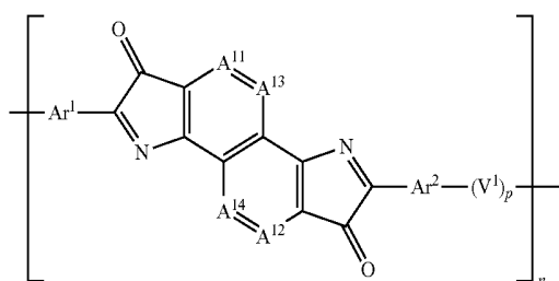
Formula (2-4)
