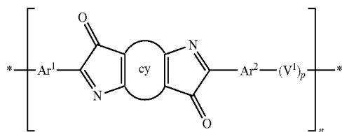
Formula (1-2B)
