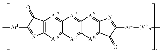
Formula (2-6)
