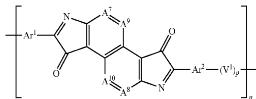
Formula (2-3)
