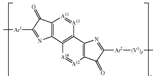
Formula (2-4)
