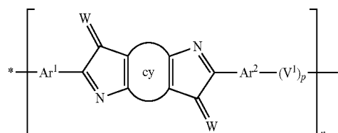
Formula (1-2')
