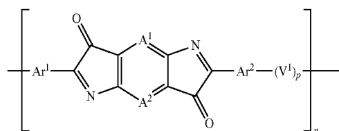
Formula (2-1)
