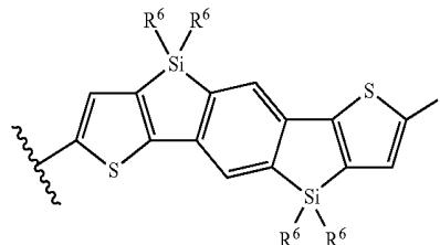
Formula (5-1)
