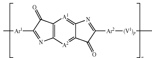
Formula (2-2)
