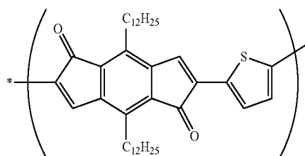
Comparative compound 3
