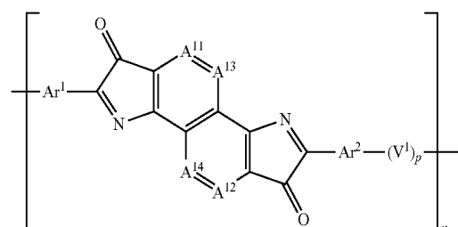
Formula (2-4)
