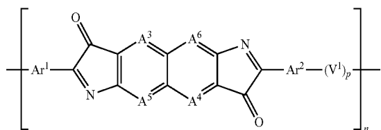
Formula (2-3)
