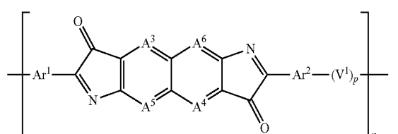
Formula (2-3)
