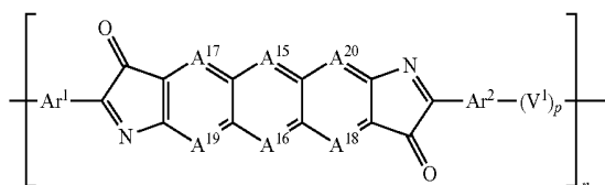
Formula (2-6)
