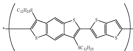
Comparative compound 4
